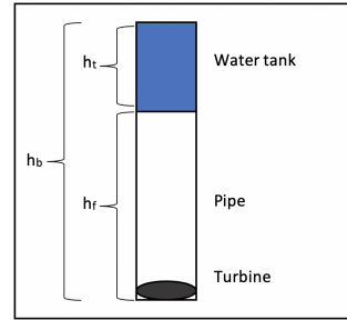
Figure 1: Shows the relation between h_b , the height of the building, h_t , the height of the tank and h_f , the height of the fall from the bottom of the tank to the turbine.
