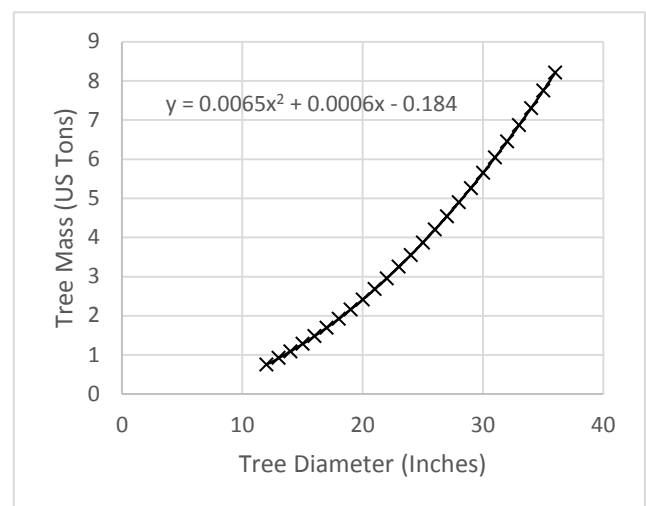
Figure 1) Tree mass as a function of diameter [3].
