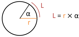
Figure 2 – Relationship between the arc length L of a circle of radius r , to the central angle \alpha in radians
