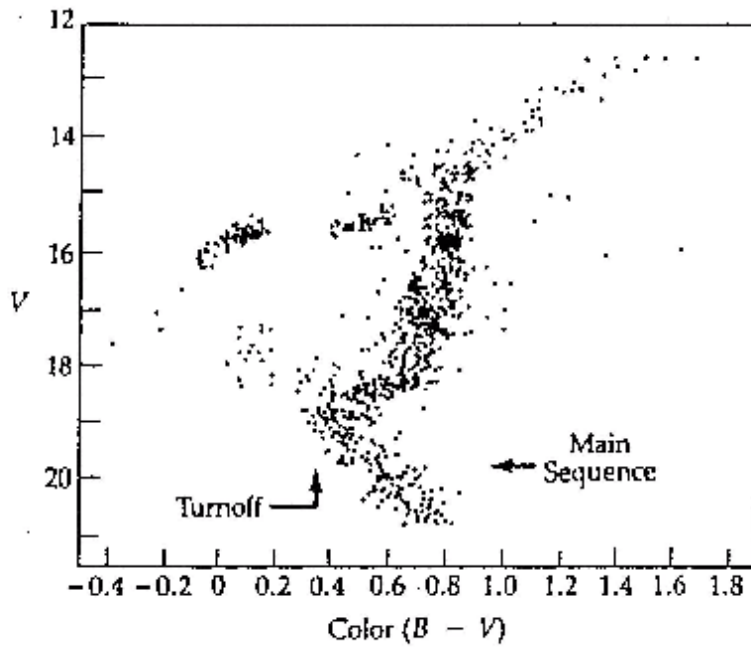
Figure 1. The HR diagram for the old star cluster NSC1
