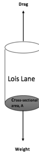
Figure 1: Diagram representing our simplistic model of the forces acting upon Lois Lane as she falls through the air.
